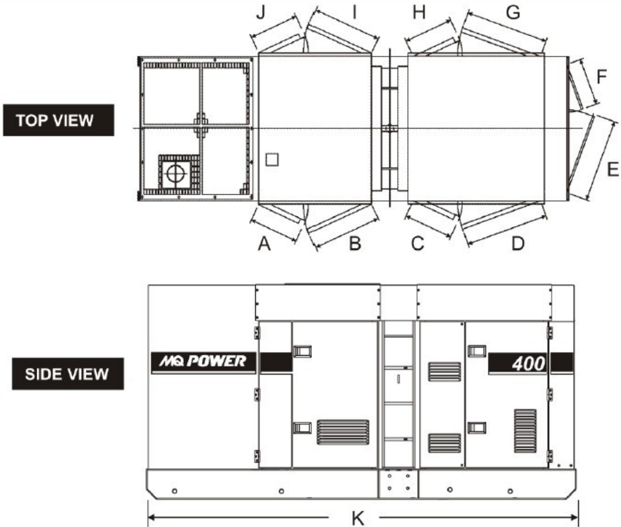
Figure 1. Dimensions
